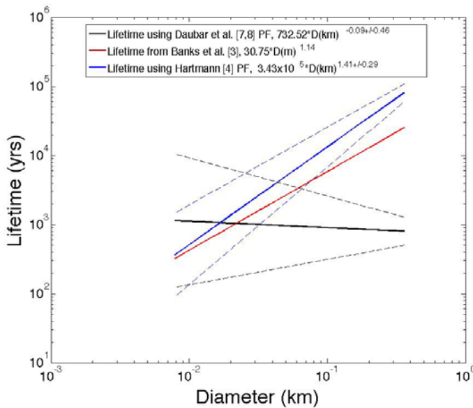
Figure 3. Lifetimes for NPLD impact craters calculated from the updated catalog using the [4] (blue) and [7,8] (black) production functions. The red line shows the lifetime function reported in [3]. The dashed lines represent the upper and lower limits of the lifetime function based on uncertainties propagated from crater counting.
