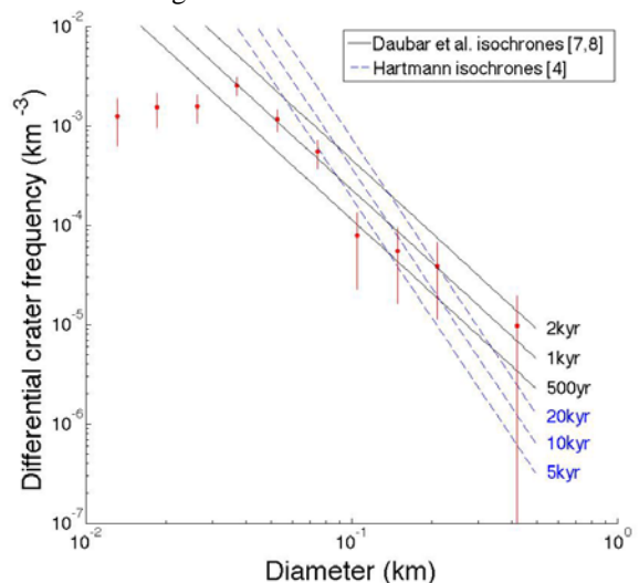
Figure 2. Differential size-frequency distribution of NPLD crater population is plotted in red. The Daubar et al. [7,8] isochrones for 0.5, 1 and 2 kyr are shown in solid black while the Hartmann [4] isochrones for 5, 10 and 20 kyr are shown in dashed blue.
